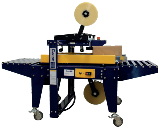
CT 102 with conveyors and castor wheels
